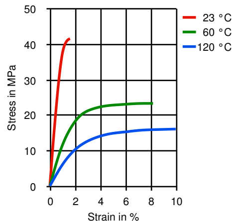
True Stress-strain
